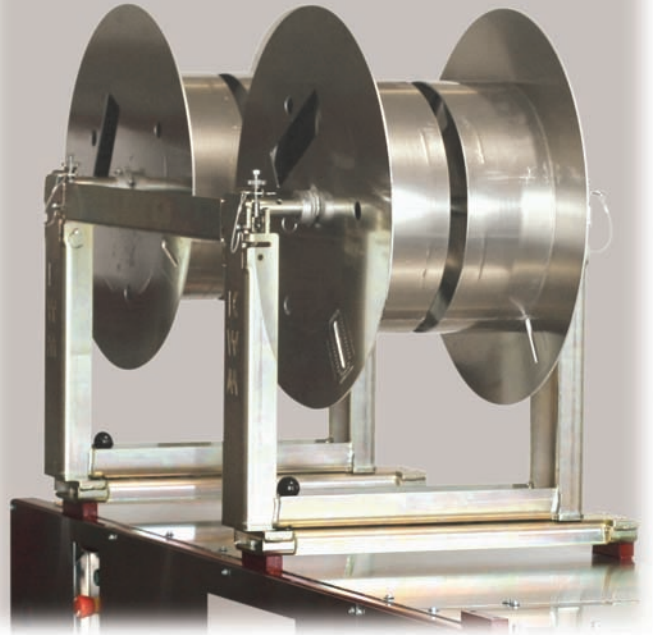
Quick release turnstile and transfer bars
